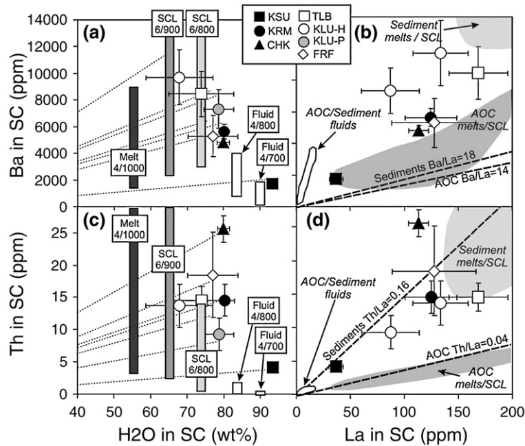
Fig. 8. Variations of \text{H}_2\text{O} , Ba, Th and La in slab components (SCs). Vertical bars (figures a and c) and shadowed fields (figures b and d) illustrate the compositions of fluids, super critical liquids (SCL) and melts equilibrated with eclogitized altered oceanic crust (AOC) and sediments [66] as calculated by using bulk part partition coefficients and major element compositions of slab fluids and melts at different P – T conditions from [56]. For example, black vertical bar labelled as “Melt 4/1000” in Ba versus \text{H}_2\text{O} diagram indicates a range of water-saturated melts with \text{H}_2\text{O} \sim 55 wt.% coexisting with eclogitized AOC (lower limit) and sediments (upper limit) at pressure 4 GPa and temperature 1000 °C. Short dashed lines in figures a and c indicate shifting SC compositions with increasing amount of solutes (Si, Al, Na, etc.). Note high Ba and Th concentrations in Kamchatka SCs, which cannot be explained by dehydration or melting of AOC and therefore imply involvement of sediment-derived melts and/or SCL.
